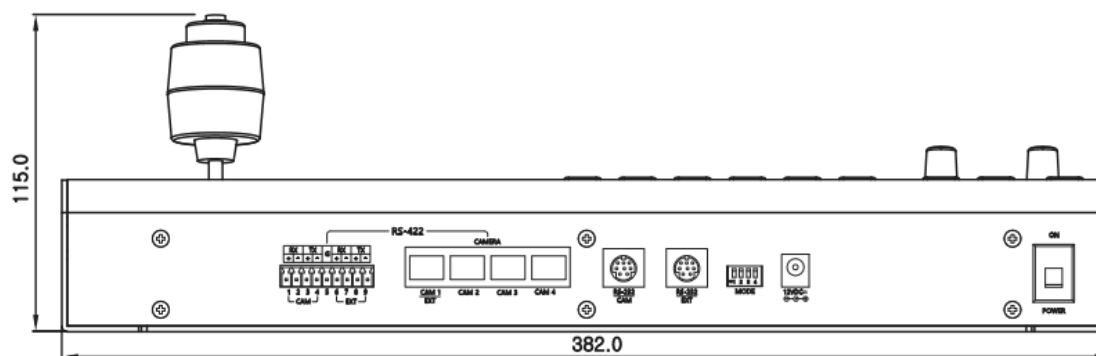
REAR View
